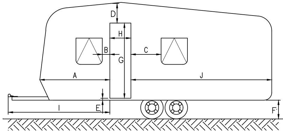
ELEVATION VIEW
